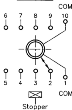
SCHEMATIC
